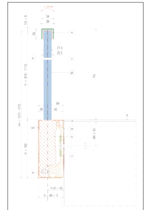
Abb. 8.61: GM RAILING® Side
