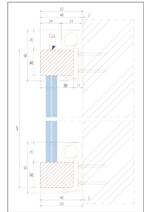
Abb. 8.64: GM WINDOORAIL®
