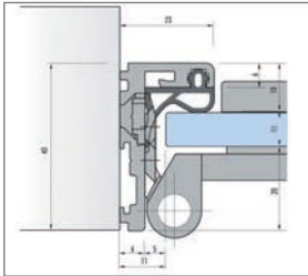
Abb. 8.49: Detail
