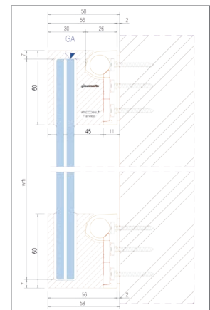
Abb. 8.65: GM WINDOORAIL® Frameless
